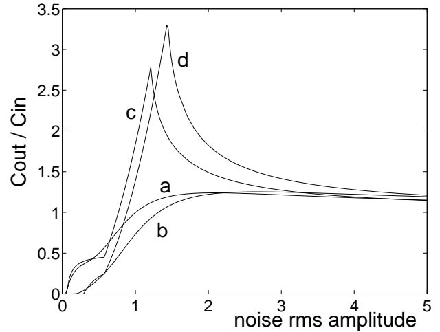
Fig. 2. Ratio of the information capacities C_{\text{out}}/C_{\text{in}} as a function of the rms amplitude of the zero-mean noise \eta_j . In (a) and (b) \eta_j is Gaussian; in (c) and (d) \eta_j is uniform. Also in (a) and (c) \theta = 1.1 ; in (b) and (d) \theta = 1.5 .
