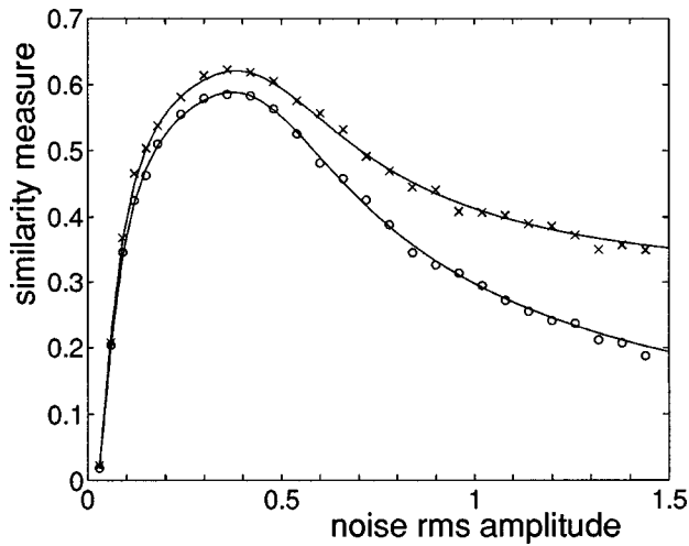
Fig. 2. Similarity between input image S(x, y) and output image Y(x, y) as a function of the input noise rms amplitude under the conditions of Fig. 1 with probability p_1 = 0.148 . Solid curves, theoretical expressions of the cross correlation R_{SY} of Eq. (7) (upper trace) and the cross covariance C_{SY} of Eq. (8) (lower trace). The two sets of discrete data points are experimental estimations through pixels counting on images.
