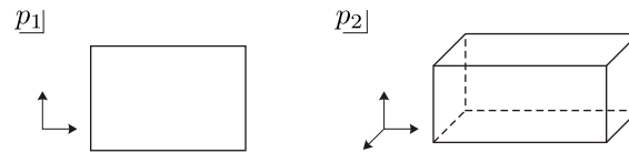
Figure 11. p_1 and p_2 are respectively examples of boxes of \mathbb{R}^2 and \mathbb{R}^3 .
