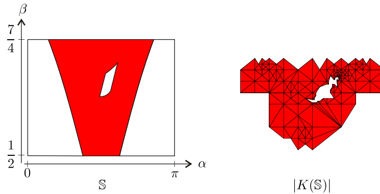
Figure 19. The feasible configuration set S and a triangulation generated by HIA.
